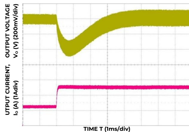
Figure 10. Transient Response to Dynamic Load Change from 50% to 100% at 12V in , C out =3x10uF+470uF, C Tune =1000pF, R Tune =30.1kΩ
