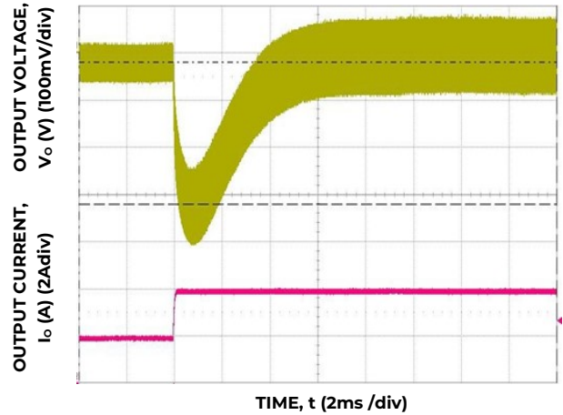
Figure 4. Transient Response to Dynamic Load Change from 50% to 100% at 12V in , C_{out}=3 \times 10\mu F + 470\mu F , C_{Tune}=1000pF , R_{Tune}=30.1k\Omega
