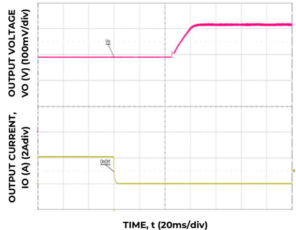
Figure 5. Typical Start-up Using On/Off Voltage ( I_o = I_{o,max} ).
