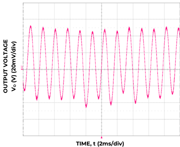
Figure 3. Typical output ripple and noise ( C_o=3 \times 10\mu F + 470\mu F , V_{IN}=12V , I_o = I_{o,max} ).
