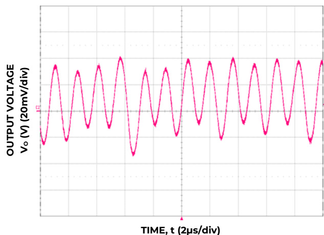
Figure 9. Typical output ripple and noise (C o =3x10uF+470uF, V IN = 12V, I o = I o,max ).
