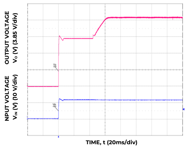
Figure 6. Typical Start-up Using Input Voltage ( V_{IN}=12V , I_o = I_o = I_{o,max} ).
