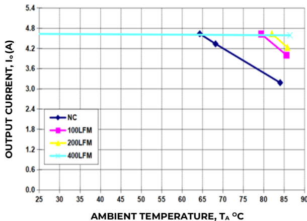
Figure 14. Derating Output Current versus Ambient Temperature and Airflow. V_{IN} = 12V
